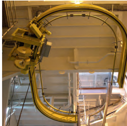
Radius going monorail trolley
