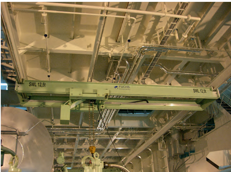
Double girder overhead crane with low headroom for engine room
