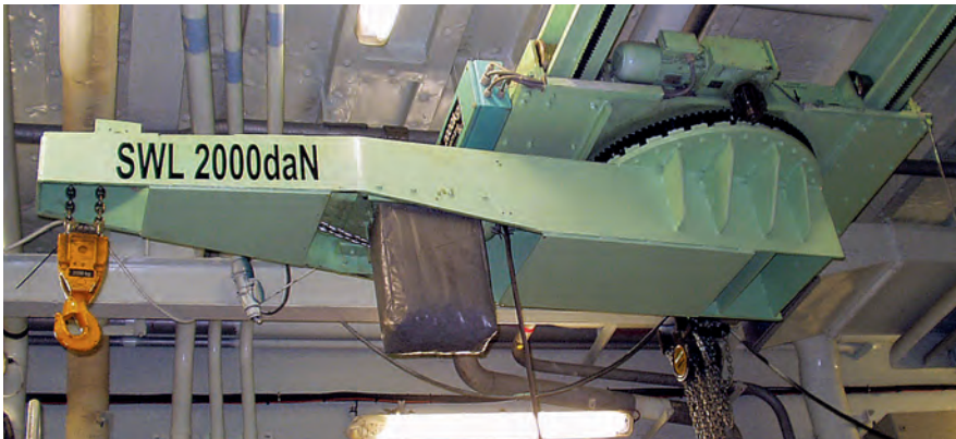
Overhead slewing jib crane for engine room
